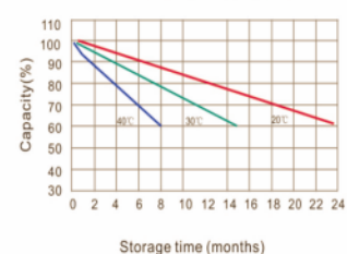
Self-discharge characteristic
