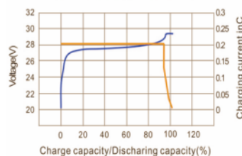
0.2C CC-CV charge characteristic
